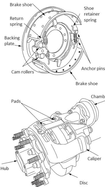
Figure 2.1 Drum and disc brake components
